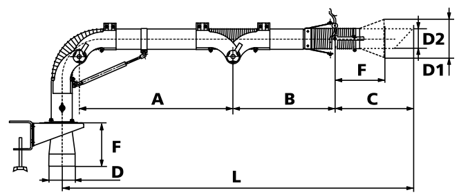
Type S (mounting over the bracket)
